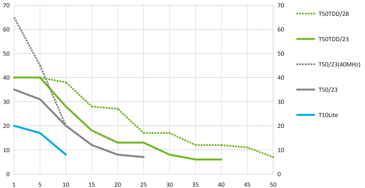
Throughput vs Distance with maximum radio Tx power, 6 dB noise margin (Mbps/km) Not legal within European Union
